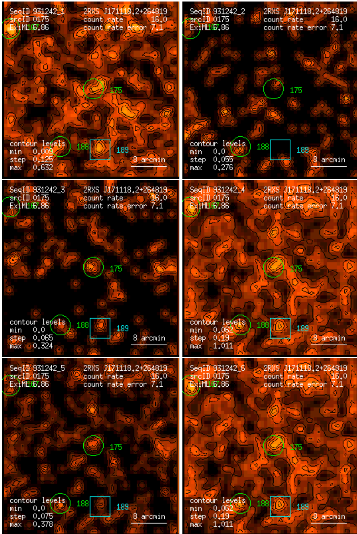
Figure 175: RASS 931242: detection 0175: band rate images, Gaussian filter: (1) PSPC channels 11 – 41, (2) 52 – 90, (3) 91 – 201, (4) 11 – 235, (5) 52 – 201, (6) 11 – 201. Broad band rates in counts/ks. Band rate contour levels in counts/ks/arcmin 2 .
