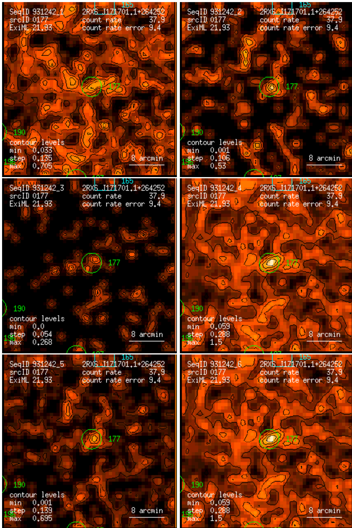
Figure 177: RASS 931242: detection 0177: band rate images, Gaussian filter: (1) PSPC channels 11 – 41, (2) 52 – 90, (3) 91 – 201, (4) 11 – 235, (5) 52 – 201, (6) 11 – 201. Broad band rates in counts/ks. Band rate contour levels in counts/ks/arcmin 2 .
