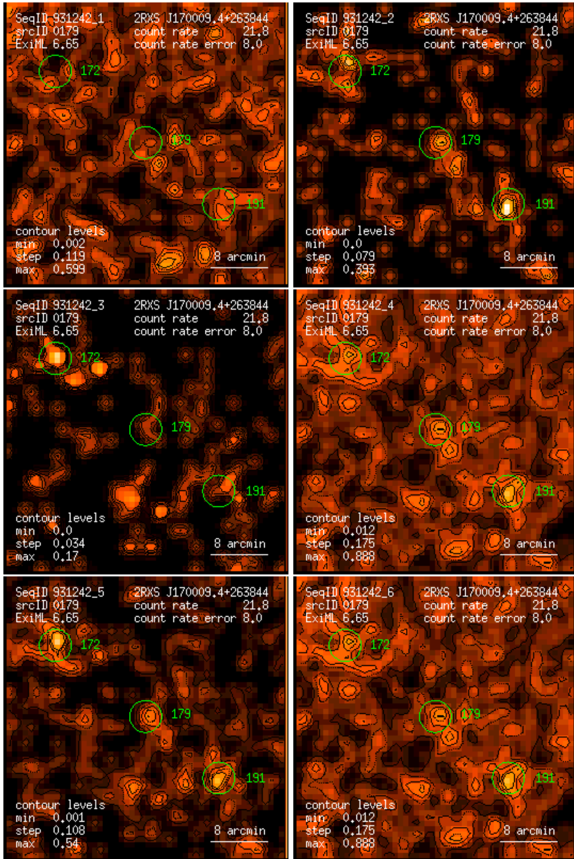
Figure 179: RASS 931242: detection 0179: band rate images, Gaussian filter: (1) PSPC channels 11 – 41, (2) 52 – 90, (3) 91 – 201, (4) 11 – 235, (5) 52 – 201, (6) 11 – 201. Broad band rates in counts/ks. Band rate contour levels in counts/ks/arcmin 2 .
