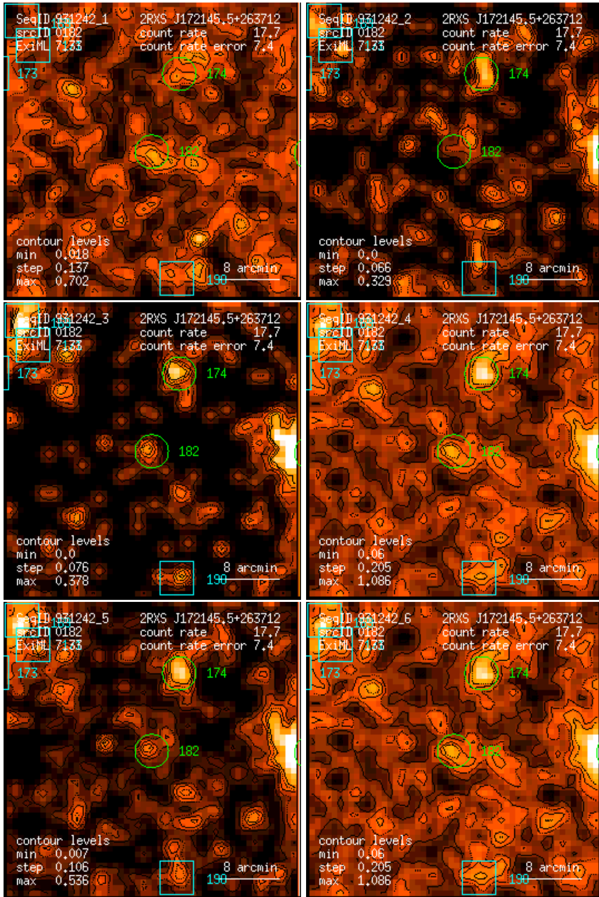
Figure 182: RASS 931242: detection 0182: band rate images, Gaussian filter: (1) PSPC channels 11 – 41, (2) 52 – 90, (3) 91 – 201, (4) 11 – 235, (5) 52 – 201, (6) 11 – 201. Broad band rates in counts/ks. Band rate contour levels in counts/ks/arcmin 2 .
