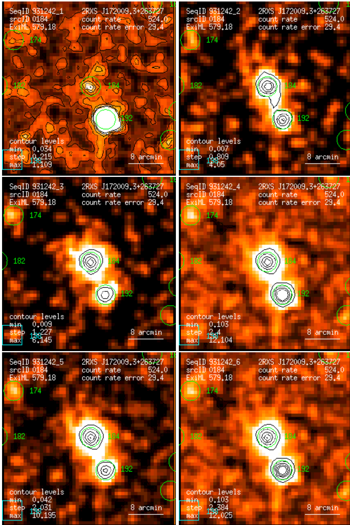
Figure 184: RASS 931242: detection 0184: band rate images, Gaussian filter: (1) PSPC channels 11 – 41, (2) 52 – 90, (3) 91 – 201, (4) 11 – 235, (5) 52 – 201, (6) 11 – 201. Broad band rates in counts/ks. Band rate contour levels in counts/ks/arcmin 2 .
