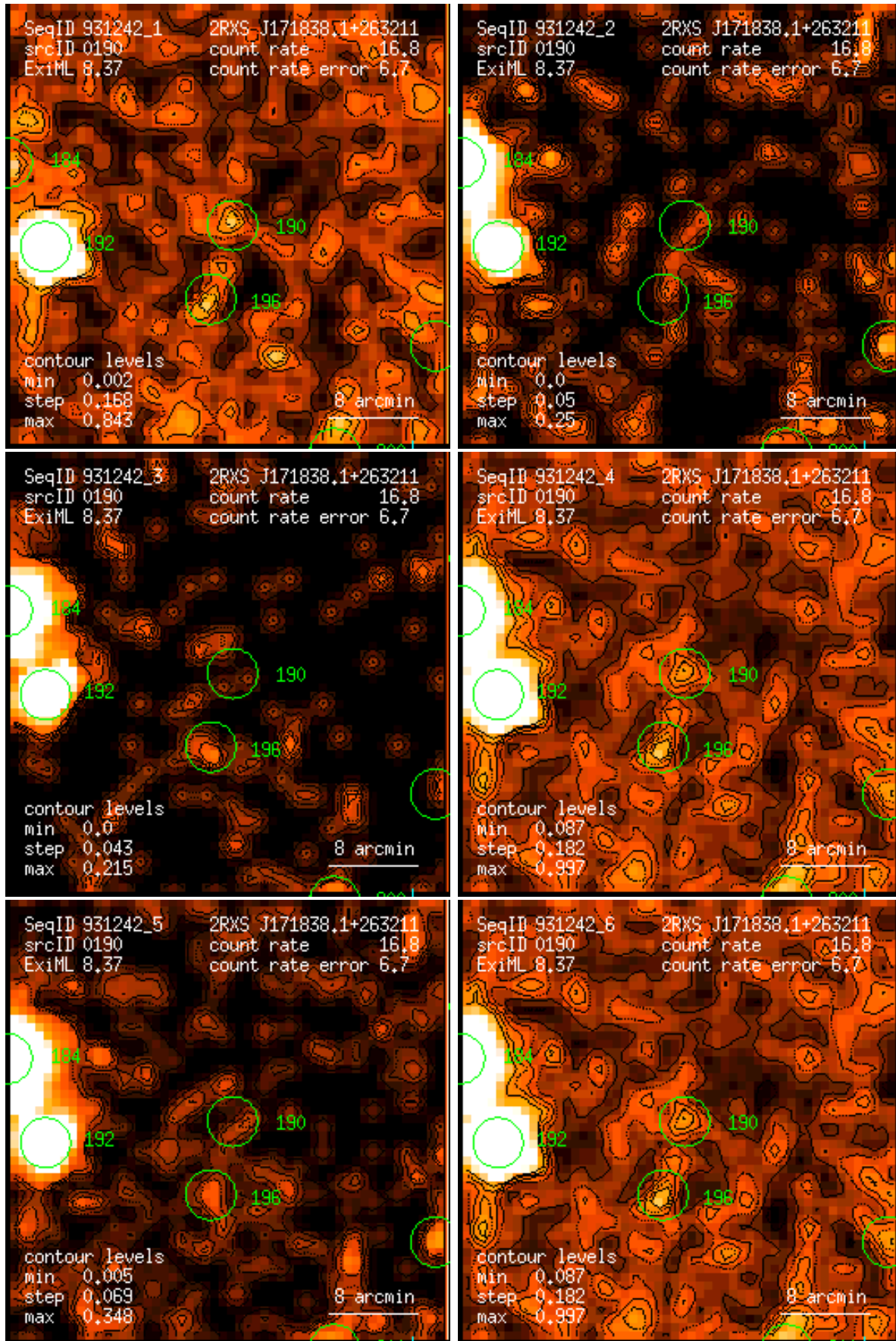
Figure 190: RASS 931242: detection 0190: band rate images, Gaussian filter: (1) PSPC channels 11 – 41, (2) 52 – 90, (3) 91 – 201, (4) 11 – 235, (5) 52 – 201, (6) 11 – 201. Broad band rates in counts/ks. Band rate contour levels in counts/ks/arcmin 2 .
