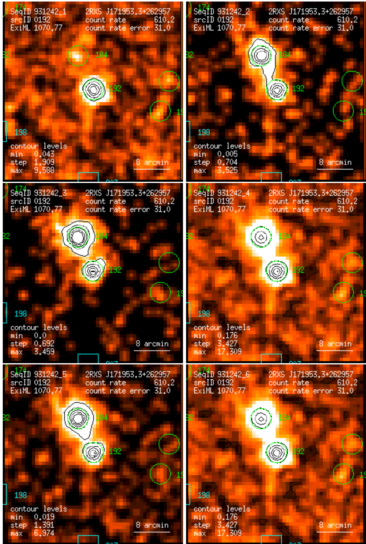
Figure 192: RASS 931242: detection 0192: band rate images, Gaussian filter: (1) PSPC channels 11 – 41, (2) 52 – 90, (3) 91 – 201, (4) 11 – 235, (5) 52 – 201, (6) 11 – 201. Broad band rates in counts/ks. Band rate contour levels in counts/ks/arcmin 2 .
