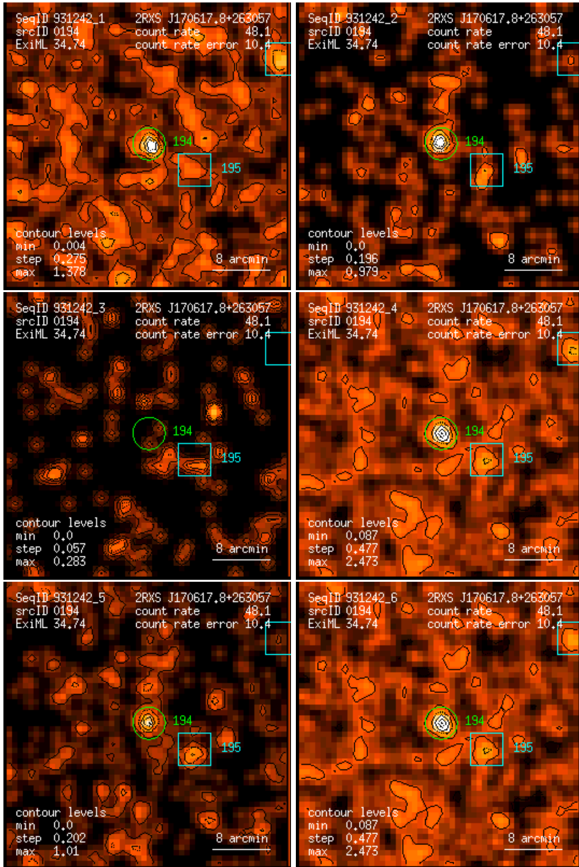
Figure 194: RASS 931242: detection 0194: band rate images, Gaussian filter: (1) PSPC channels 11 – 41, (2) 52 – 90, (3) 91 – 201, (4) 11 – 235, (5) 52 – 201, (6) 11 – 201. Broad band rates in counts/ks. Band rate contour levels in counts/ks/arcmin 2 .
