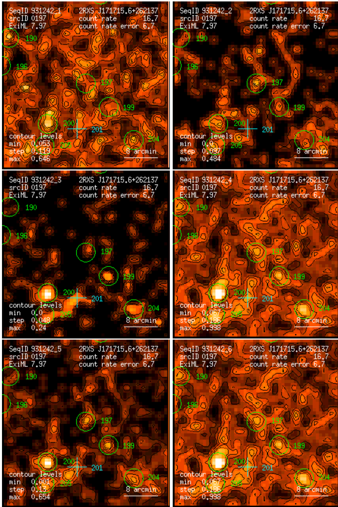
Figure 197: RASS 931242: detection 0197: band rate images, Gaussian filter: (1) PSPC channels 11 – 41, (2) 52 – 90, (3) 91 – 201, (4) 11 – 235, (5) 52 – 201, (6) 11 – 201. Broad band rates in counts/ks. Band rate contour levels in counts/ks/arcmin 2 .
