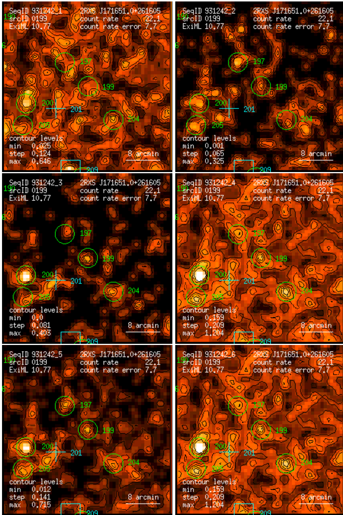
Figure 199: RASS 931242: detection 0199: band rate images, Gaussian filter: (1) PSPC channels 11 – 41, (2) 52 – 90, (3) 91 – 201, (4) 11 – 235, (5) 52 – 201, (6) 11 – 201. Broad band rates in counts/ks. Band rate contour levels in counts/ks/arcmin 2 .
