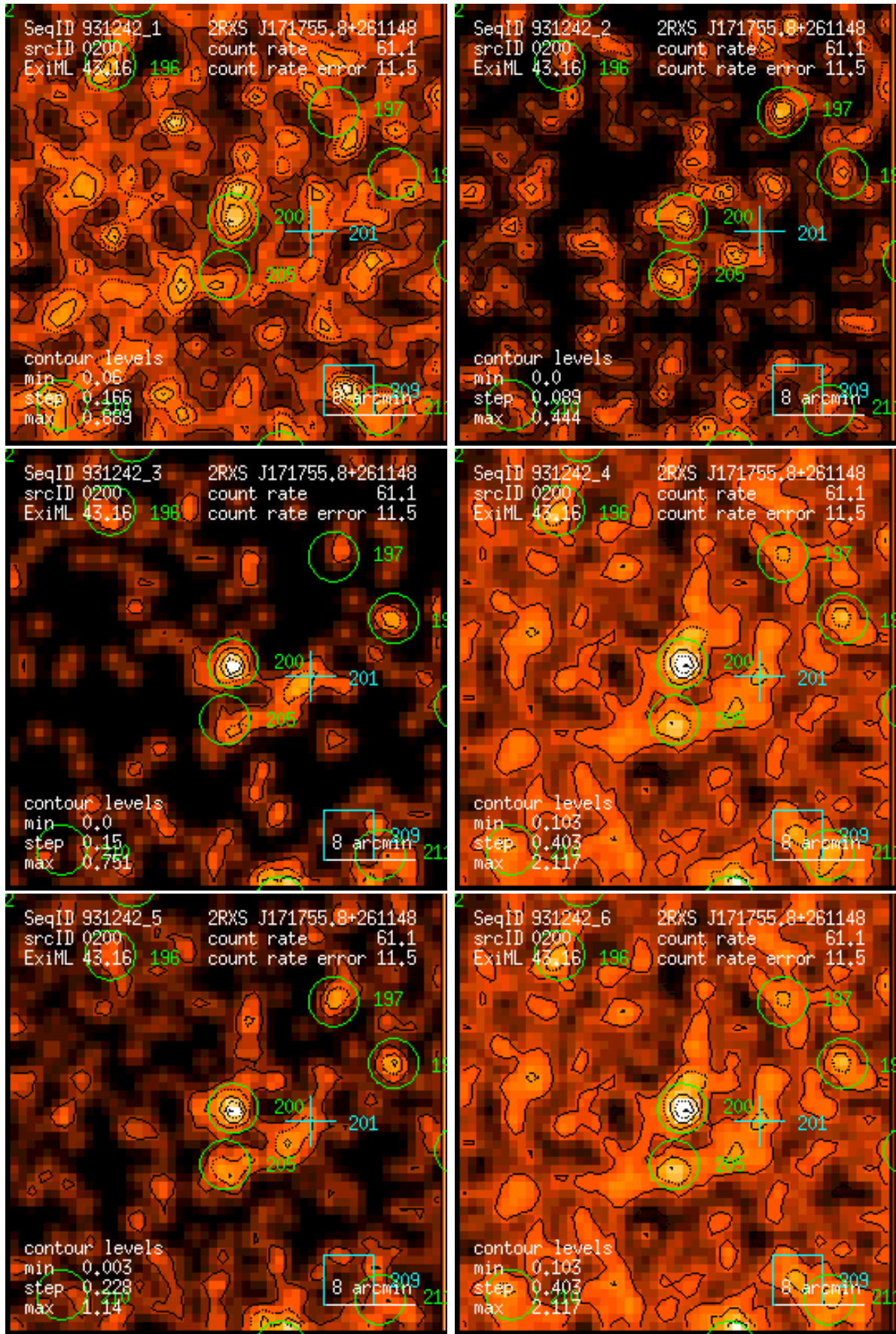
Figure 200: RASS 931242: detection 0200: band rate images, Gaussian filter: (1) PSPC channels 11 – 41, (2) 52 – 90, (3) 91 – 201, (4) 11 – 235, (5) 52 – 201, (6) 11 – 201. Broad band rates in counts/ks. Band rate contour levels in counts/ks/arcmin 2 .
