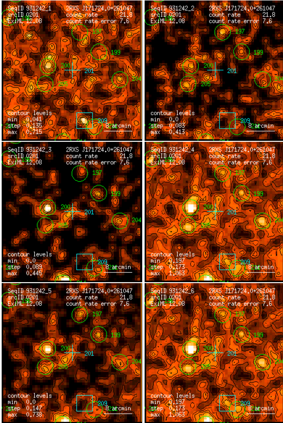
Figure 201: RASS 931242: detection 0201: band rate images, Gaussian filter: (1) PSPC channels 11 – 41, (2) 52 – 90, (3) 91 – 201, (4) 11 – 235, (5) 52 – 201, (6) 11 – 201. Broad band rates in counts/ks. Band rate contour levels in counts/ks/arcmin 2 .
