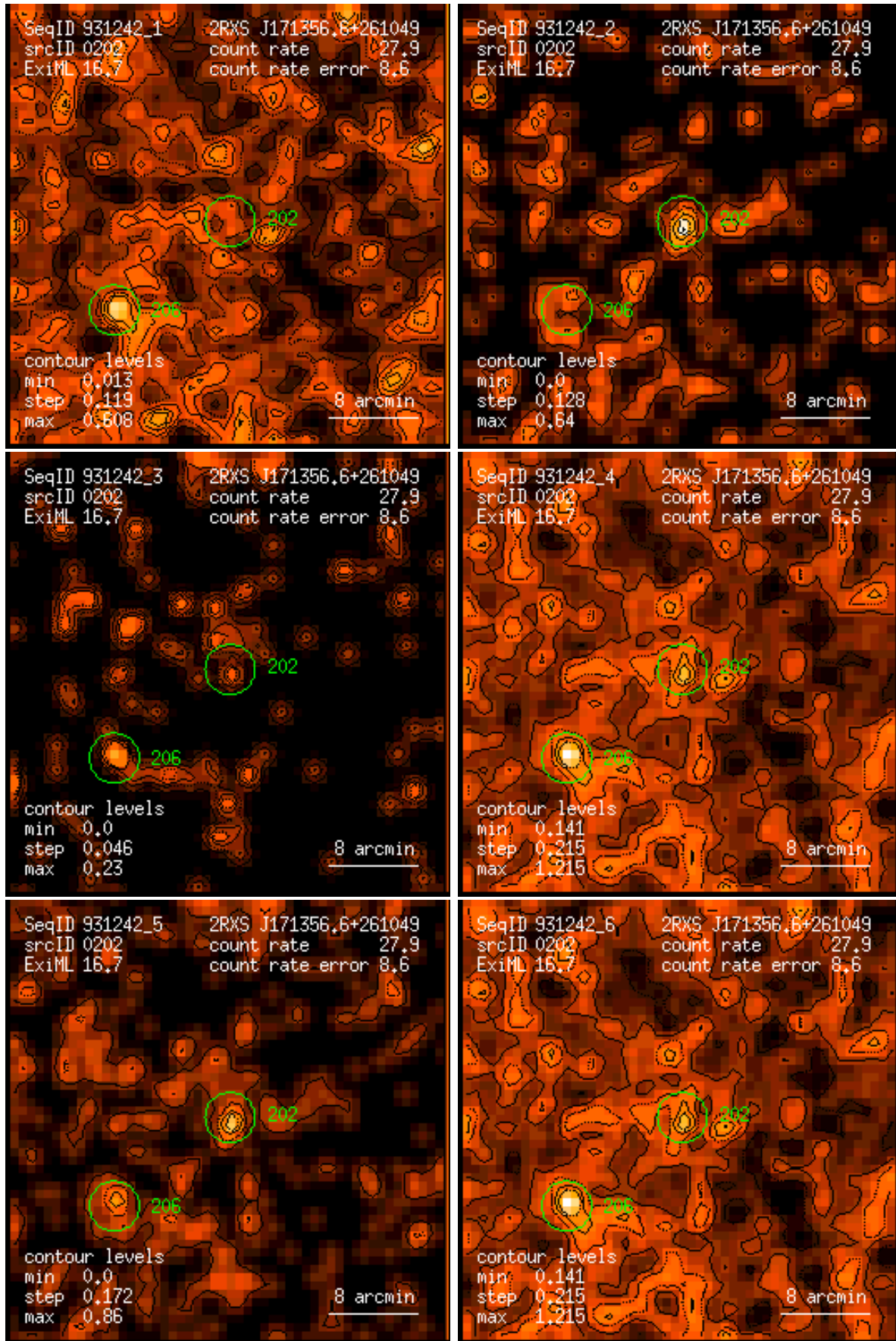
Figure 202: RASS 931242: detection 0202: band rate images, Gaussian filter: (1) PSPC channels 11 – 41, (2) 52 – 90, (3) 91 – 201, (4) 11 – 235, (5) 52 – 201, (6) 11 – 201. Broad band rates in counts/ks. Band rate contour levels in counts/ks/arcmin 2 .
