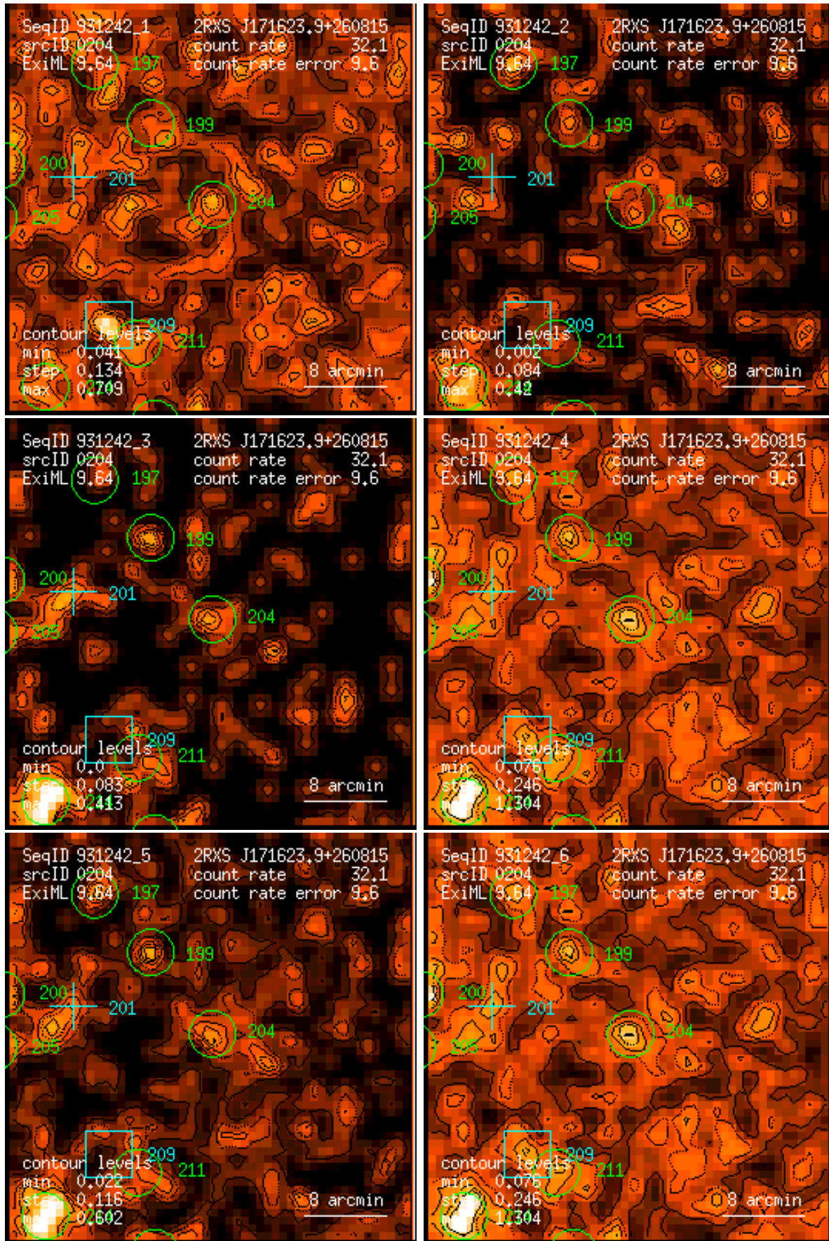
Figure 204: RASS 931242: detection 0204: band rate images, Gaussian filter: (1) PSPC channels 11 – 41, (2) 52 – 90, (3) 91 – 201, (4) 11 – 235, (5) 52 – 201, (6) 11 – 201. Broad band rates in counts/ks. Band rate contour levels in counts/ks/arcmin 2 .
