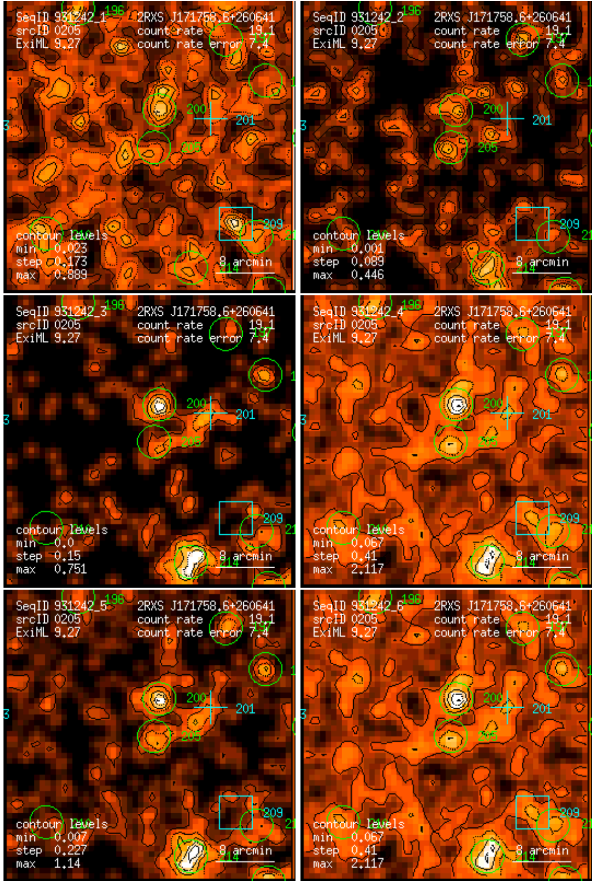
Figure 205: RASS 931242: detection 0205: band rate images, Gaussian filter: (1) PSPC channels 11 – 41, (2) 52 – 90, (3) 91 – 201, (4) 11 – 235, (5) 52 – 201, (6) 11 – 201. Broad band rates in counts/ks. Band rate contour levels in counts/ks/arcmin 2 .
