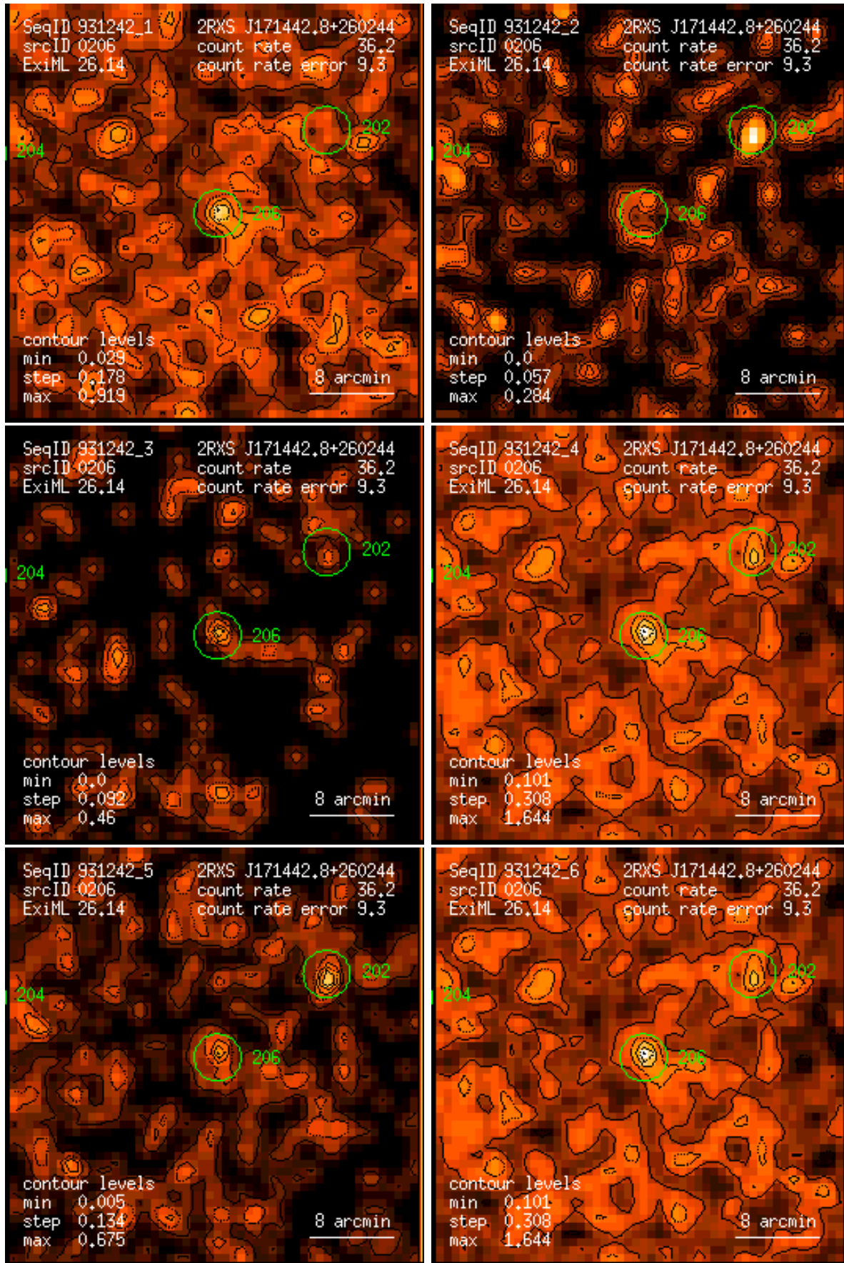
Figure 206: RASS 931242: detection 0206: band rate images, Gaussian filter: (1) PSPC channels 11 – 41, (2) 52 – 90, (3) 91 – 201, (4) 11 – 235, (5) 52 – 201, (6) 11 – 201. Broad band rates in counts/ks. Band rate contour levels in counts/ks/arcmin 2 .
