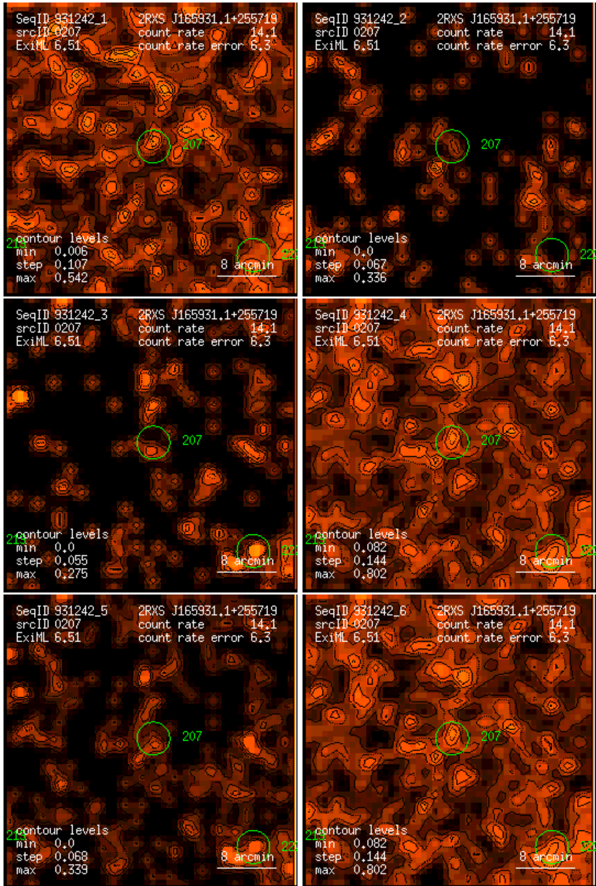
Figure 207: RASS 931242: detection 0207: band rate images, Gaussian filter: (1) PSPC channels 11 – 41, (2) 52 – 90, (3) 91 – 201, (4) 11 – 235, (5) 52 – 201, (6) 11 – 201. Broad band rates in counts/ks. Band rate contour levels in counts/ks/arcmin 2 .
