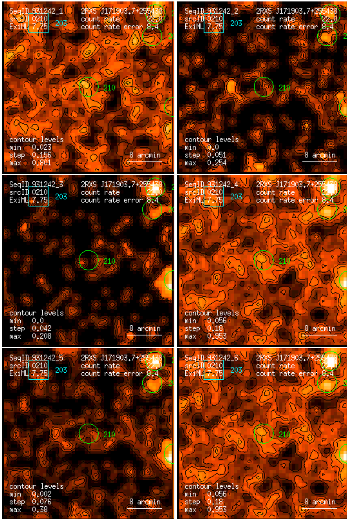
Figure 210: RASS 931242: detection 0210: band rate images, Gaussian filter: (1) PSPC channels 11 – 41, (2) 52 – 90, (3) 91 – 201, (4) 11 – 235, (5) 52 – 201, (6) 11 – 201. Broad band rates in counts/ks. Band rate contour levels in counts/ks/arcmin 2 .
