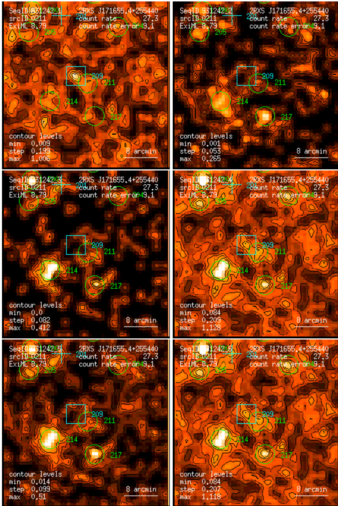
Figure 211: RASS 931242: detection 0211: band rate images, Gaussian filter: (1) PSPC channels 11 – 41, (2) 52 – 90, (3) 91 – 201, (4) 11 – 235, (5) 52 – 201, (6) 11 – 201. Broad band rates in counts/ks. Band rate contour levels in counts/ks/arcmin 2 .
