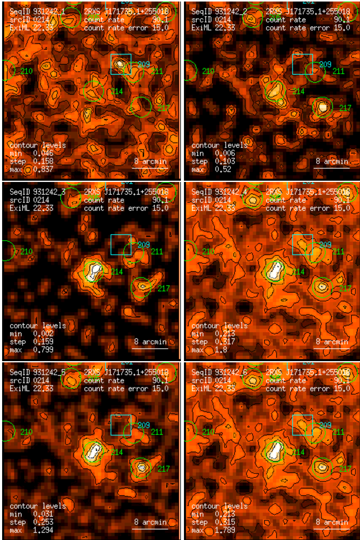
Figure 214: RASS 931242: detection 0214: band rate images, Gaussian filter: (1) PSPC channels 11 – 41, (2) 52 – 90, (3) 91 – 201, (4) 11 – 235, (5) 52 – 201, (6) 11 – 201. Broad band rates in counts/ks. Band rate contour levels in counts/ks/arcmin 2 .
