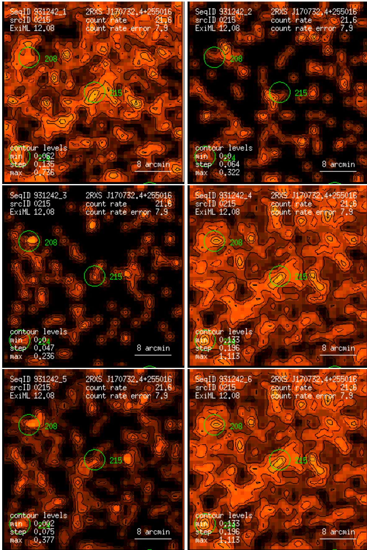
Figure 215: RASS 931242: detection 0215: band rate images, Gaussian filter: (1) PSPC channels 11 – 41, (2) 52 – 90, (3) 91 – 201, (4) 11 – 235, (5) 52 – 201, (6) 11 – 201. Broad band rates in counts/ks. Band rate contour levels in counts/ks/arcmin 2 .
