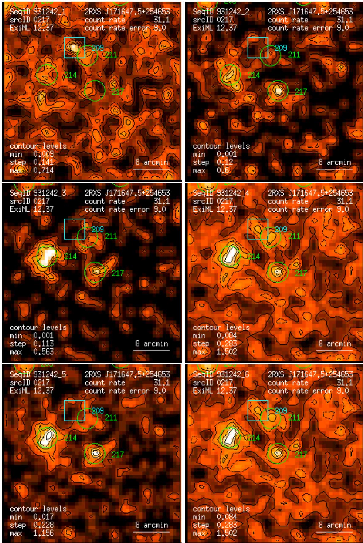
Figure 217: RASS 931242: detection 0217: band rate images, Gaussian filter: (1) PSPC channels 11 – 41, (2) 52 – 90, (3) 91 – 201, (4) 11 – 235, (5) 52 – 201, (6) 11 – 201. Broad band rates in counts/ks. Band rate contour levels in counts/ks/arcmin 2 .
