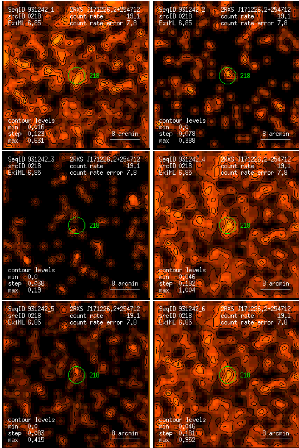
Figure 218: RASS 931242: detection 0218: band rate images, Gaussian filter: (1) PSPC channels 11 – 41, (2) 52 – 90, (3) 91 – 201, (4) 11 – 235, (5) 52 – 201, (6) 11 – 201. Broad band rates in counts/ks. Band rate contour levels in counts/ks/arcmin 2 .
