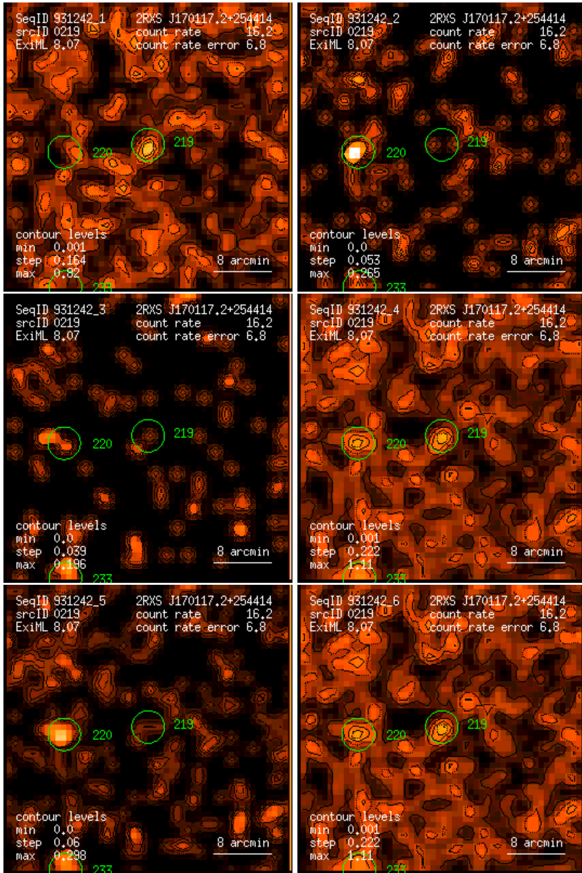
Figure 219: RASS 931242: detection 0219: band rate images, Gaussian filter: (1) PSPC channels 11 – 41, (2) 52 – 90, (3) 91 – 201, (4) 11 – 235, (5) 52 – 201, (6) 11 – 201. Broad band rates in counts/ks. Band rate contour levels in counts/ks/arcmin 2 .
