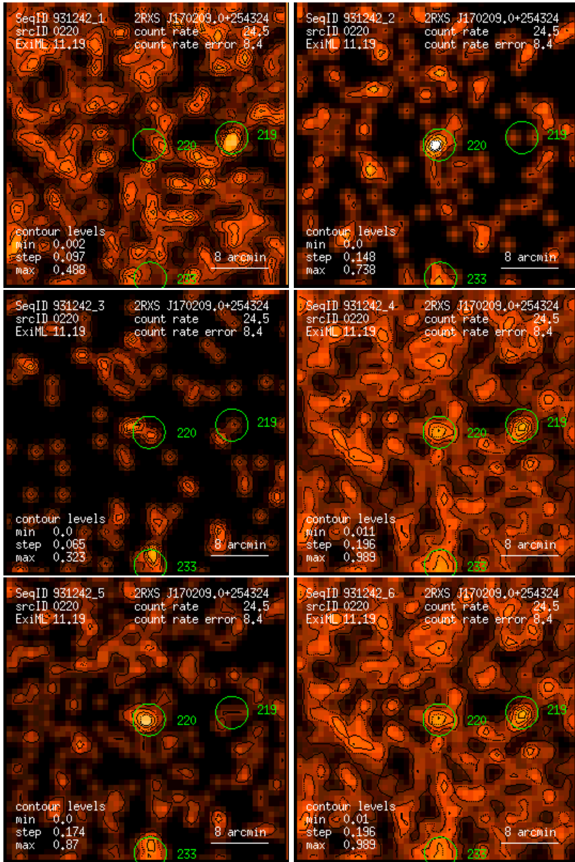
Figure 220: RASS 931242: detection 0220: band rate images, Gaussian filter: (1) PSPC channels 11 – 41, (2) 52 – 90, (3) 91 – 201, (4) 11 – 235, (5) 52 – 201, (6) 11 – 201. Broad band rates in counts/ks. Band rate contour levels in counts/ks/arcmin 2 .
