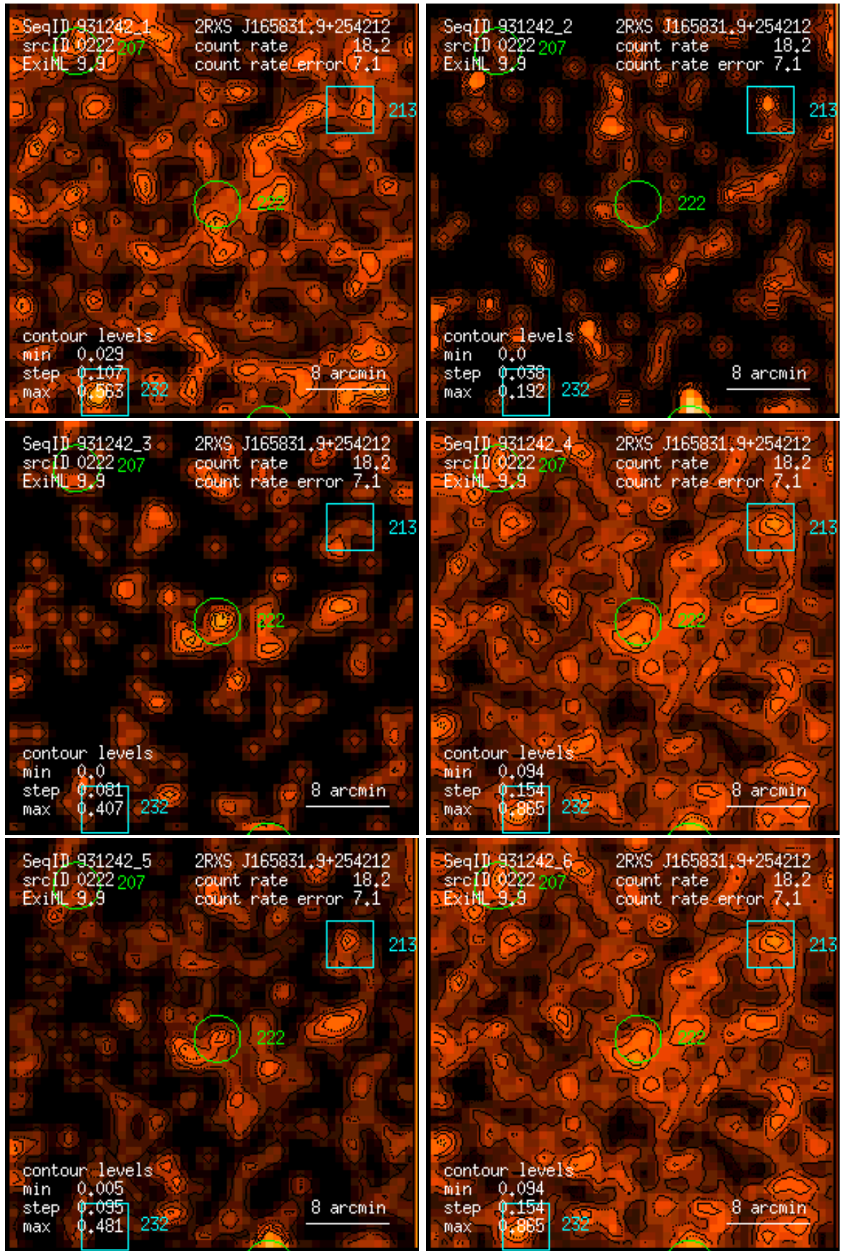
Figure 222: RASS 931242: detection 0222: band rate images, Gaussian filter: (1) PSPC channels 11 – 41, (2) 52 – 90, (3) 91 – 201, (4) 11 – 235, (5) 52 – 201, (6) 11 – 201. Broad band rates in counts/ks. Band rate contour levels in counts/ks/arcmin 2 .
