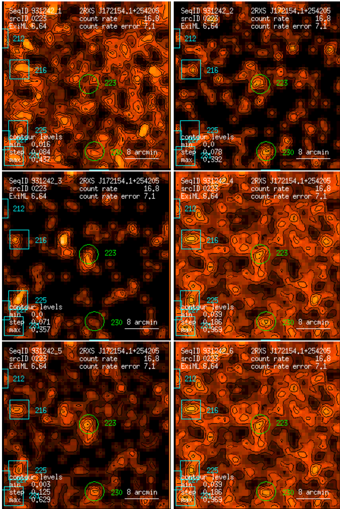
Figure 223: RASS 931242: detection 0223: band rate images, Gaussian filter: (1) PSPC channels 11 – 41, (2) 52 – 90, (3) 91 – 201, (4) 11 – 235, (5) 52 – 201, (6) 11 – 201. Broad band rates in counts/ks. Band rate contour levels in counts/ks/arcmin 2 .
