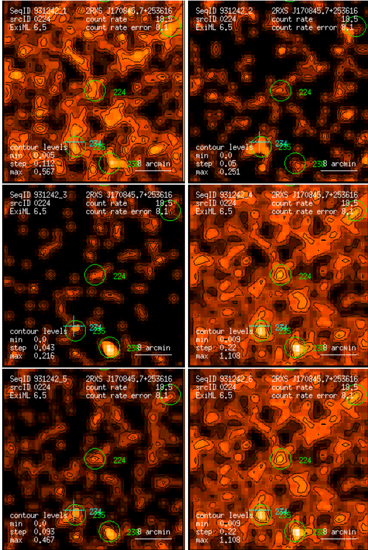
Figure 224: RASS 931242: detection 0224: band rate images, Gaussian filter: (1) PSPC channels 11 – 41, (2) 52 – 90, (3) 91 – 201, (4) 11 – 235, (5) 52 – 201, (6) 11 – 201. Broad band rates in counts/ks. Band rate contour levels in counts/ks/arcmin 2 .
