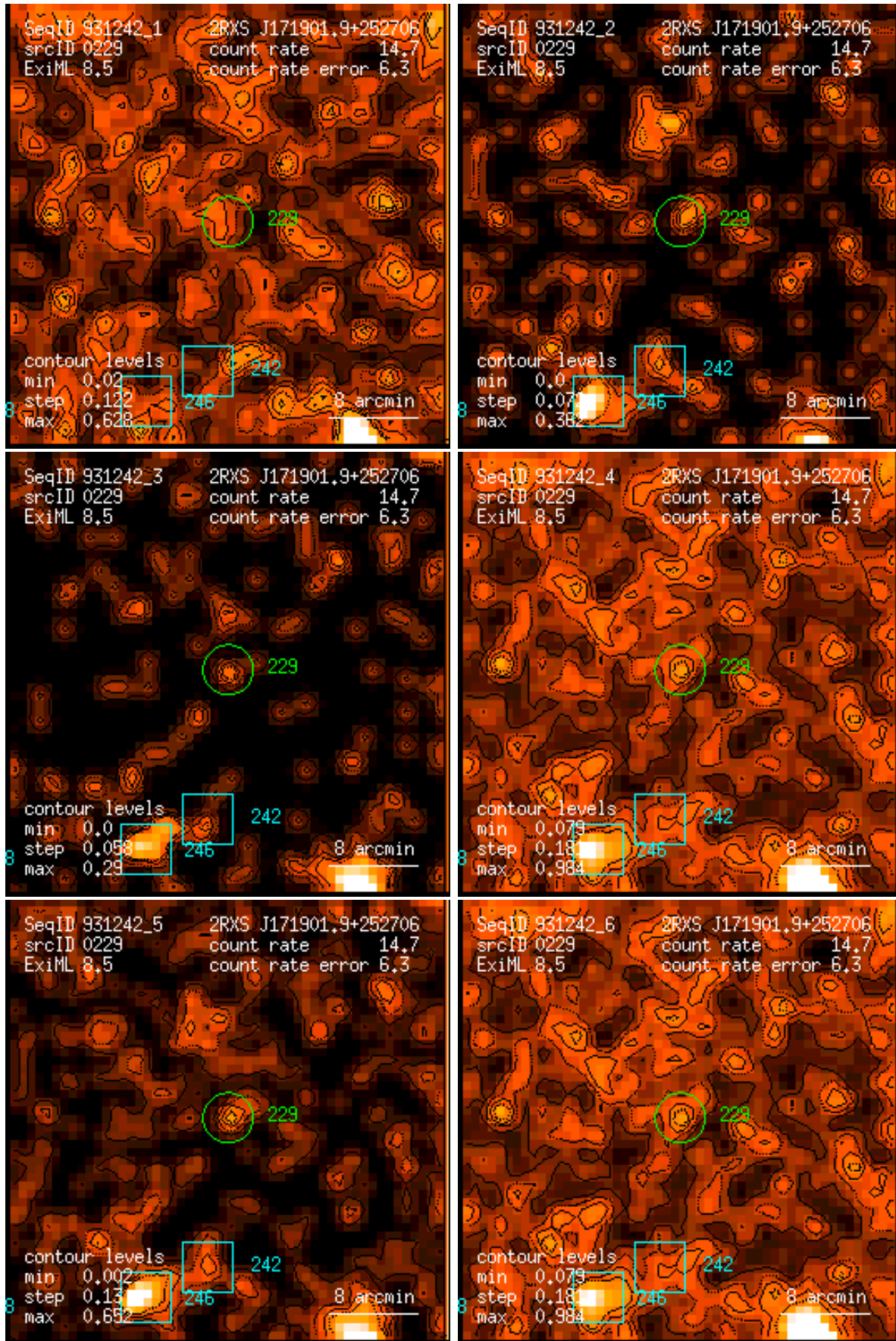
Figure 229: RASS 931242: detection 0229: band rate images, Gaussian filter: (1) PSPC channels 11 – 41, (2) 52 – 90, (3) 91 – 201, (4) 11 – 235, (5) 52 – 201, (6) 11 – 201. Broad band rates in counts/ks. Band rate contour levels in counts/ks/arcmin 2 .
