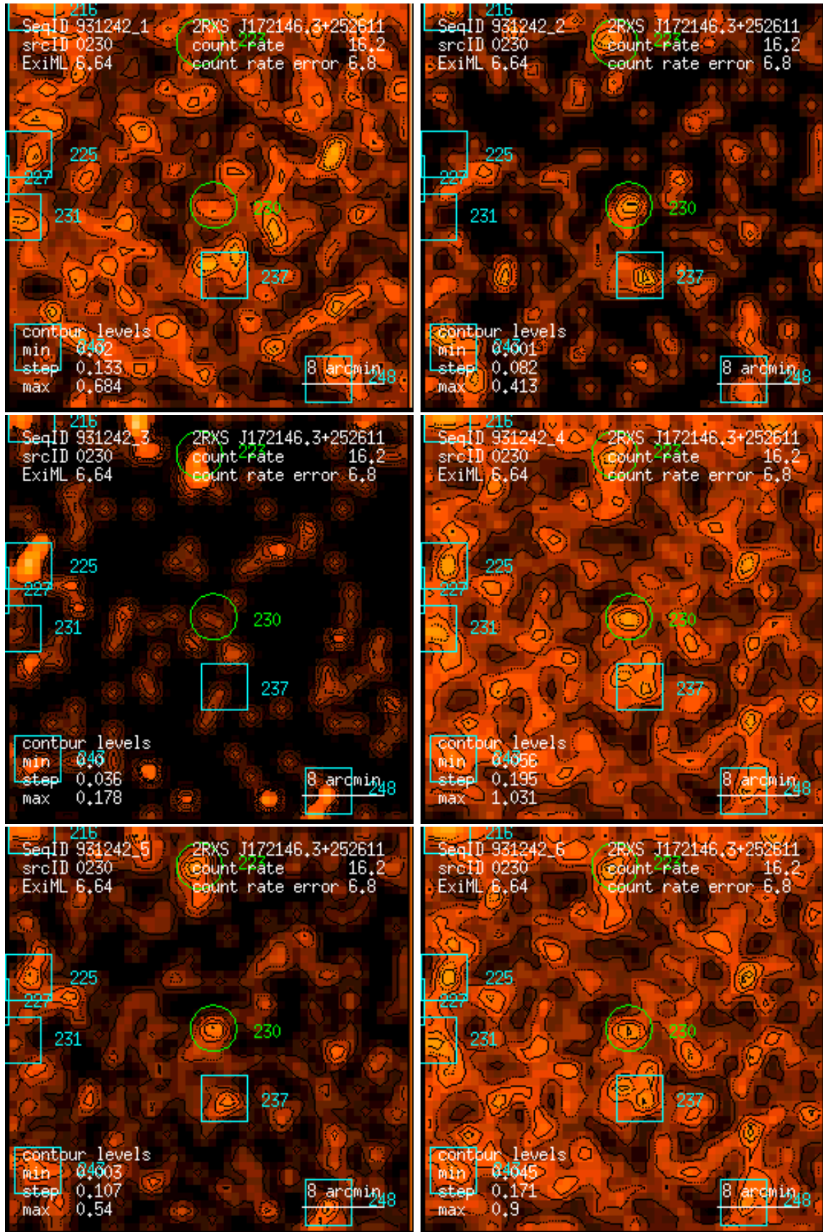
Figure 230: RASS 931242: detection 0230: band rate images, Gaussian filter: (1) PSPC channels 11 – 41, (2) 52 – 90, (3) 91 – 201, (4) 11 – 235, (5) 52 – 201, (6) 11 – 201. Broad band rates in counts/ks. Band rate contour levels in counts/ks/arcmin 2 .
