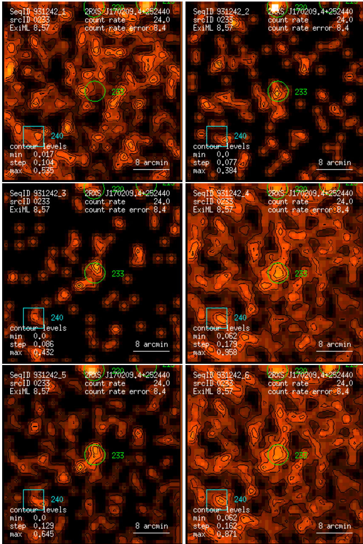
Figure 233: RASS 931242: detection 0233: band rate images, Gaussian filter: (1) PSPC channels 11 – 41, (2) 52 – 90, (3) 91 – 201, (4) 11 – 235, (5) 52 – 201, (6) 11 – 201. Broad band rates in counts/ks. Band rate contour levels in counts/ks/arcmin 2 .
