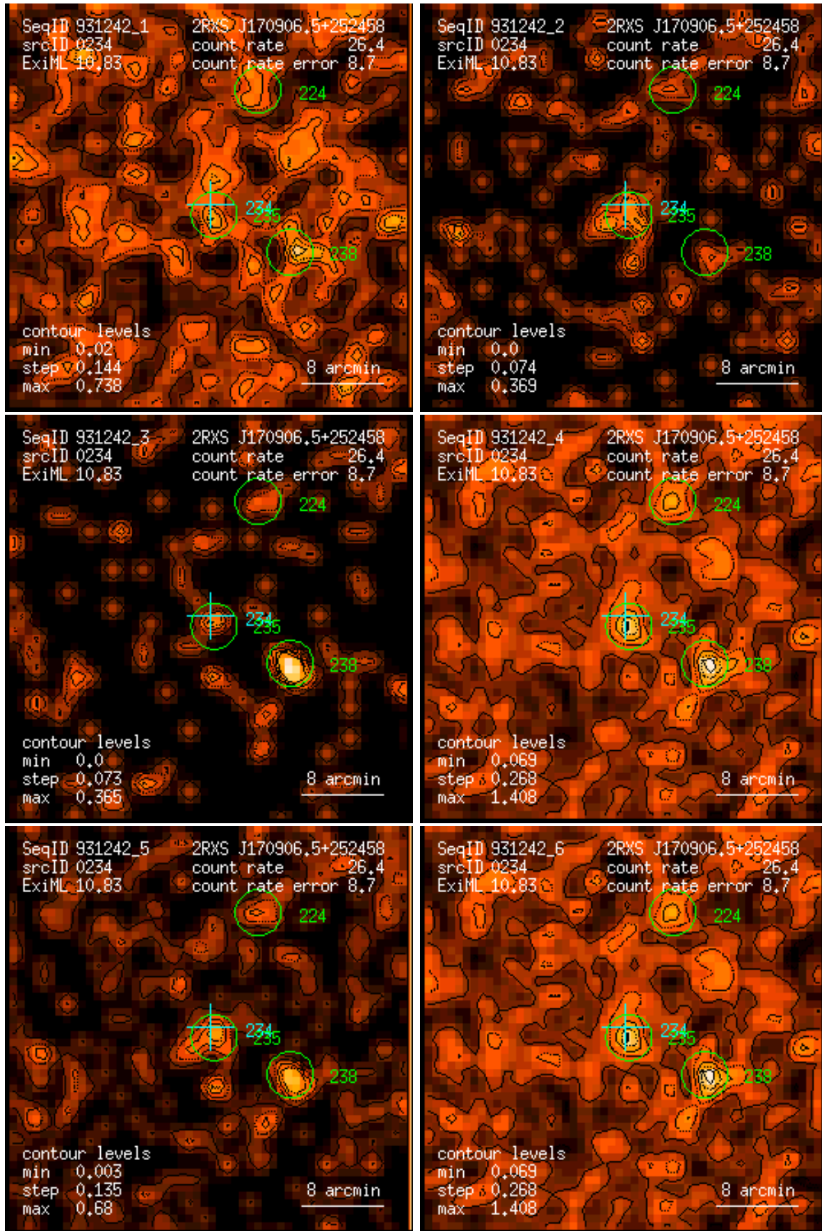
Figure 234: RASS 931242: detection 0234: band rate images, Gaussian filter: (1) PSPC channels 11 – 41, (2) 52 – 90, (3) 91 – 201, (4) 11 – 235, (5) 52 – 201, (6) 11 – 201. Broad band rates in counts/ks. Band rate contour levels in counts/ks/arcmin 2 .
