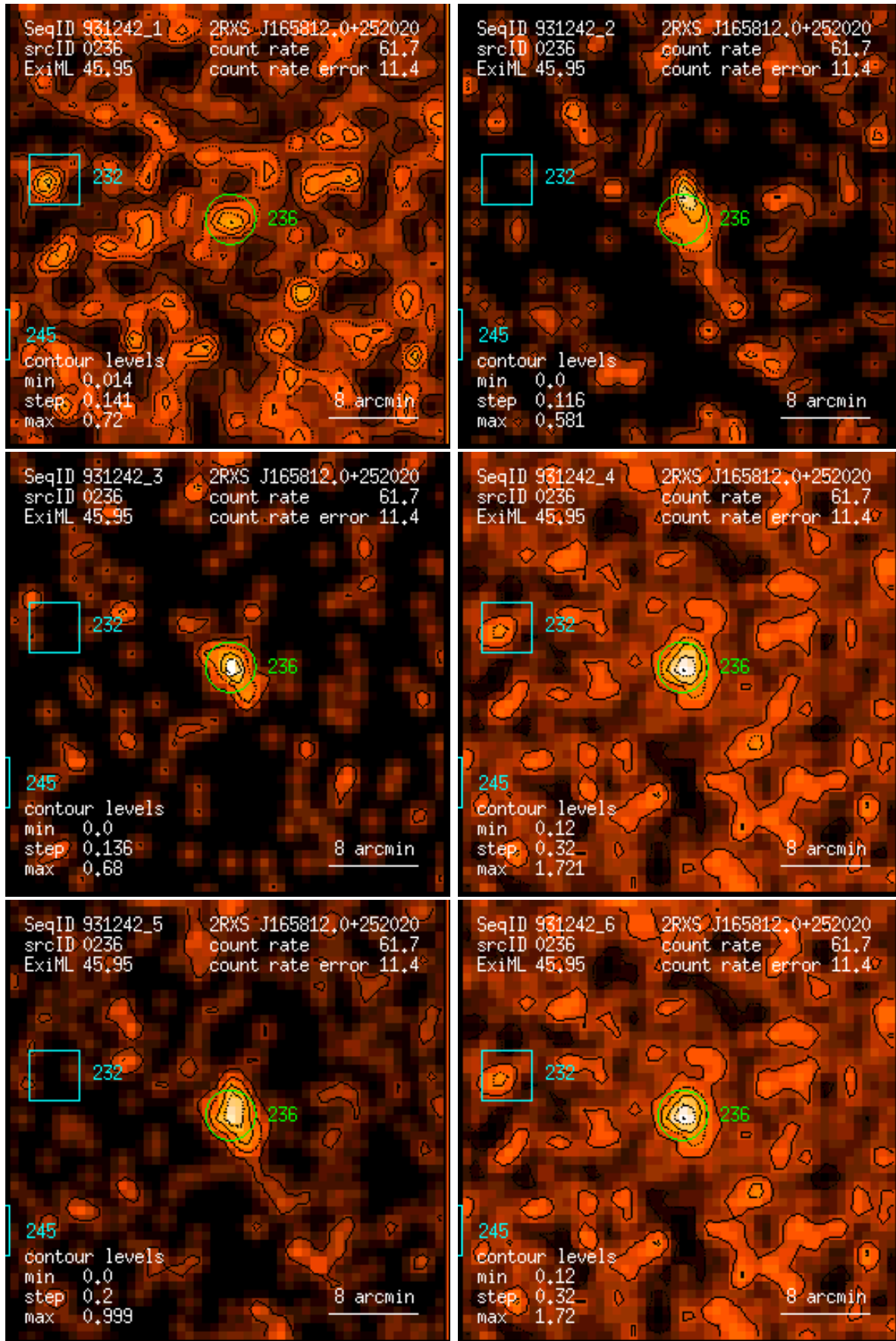
Figure 236: RASS 931242: detection 0236: band rate images, Gaussian filter: (1) PSPC channels 11 – 41, (2) 52 – 90, (3) 91 – 201, (4) 11 – 235, (5) 52 – 201, (6) 11 – 201. Broad band rates in counts/ks. Band rate contour levels in counts/ks/arcmin 2 .
