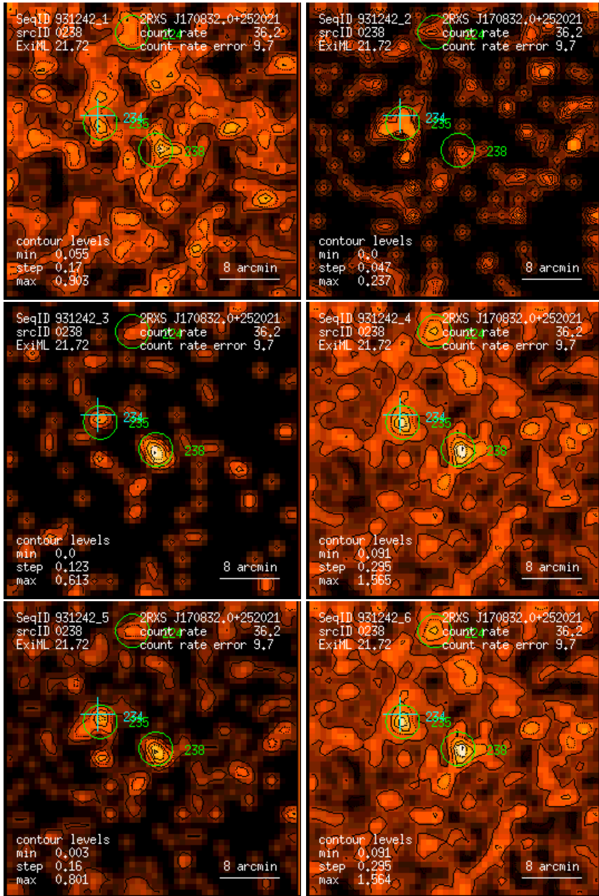
Figure 238: RASS 931242: detection 0238: band rate images, Gaussian filter: (1) PSPC channels 11 – 41, (2) 52 – 90, (3) 91 – 201, (4) 11 – 235, (5) 52 – 201, (6) 11 – 201. Broad band rates in counts/ks. Band rate contour levels in counts/ks/arcmin 2 .
