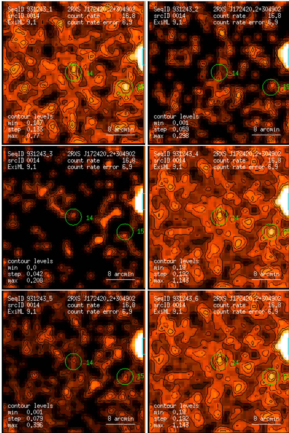
Figure 14: RASS 931243: detection 0014: band rate images, Gaussian filter: (1) PSPC channels 11 – 41, (2) 52 – 90, (3) 91 – 201, (4) 11 – 235, (5) 52 – 201, (6) 11 – 201. Broad band rates in counts/ks. Band rate contour levels in counts/ks/arcmin 2 .
