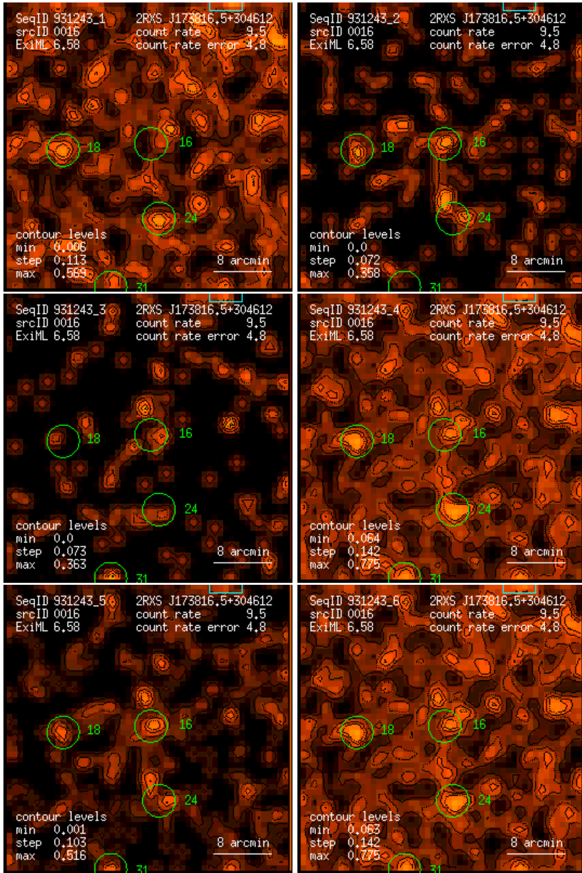
Figure 16: RASS 931243: detection 0016: band rate images, Gaussian filter: (1) PSPC channels 11 – 41, (2) 52 – 90, (3) 91 – 201, (4) 11 – 235, (5) 52 – 201, (6) 11 – 201. Broad band rates in counts/ks. Band rate contour levels in counts/ks/arcmin 2 .
