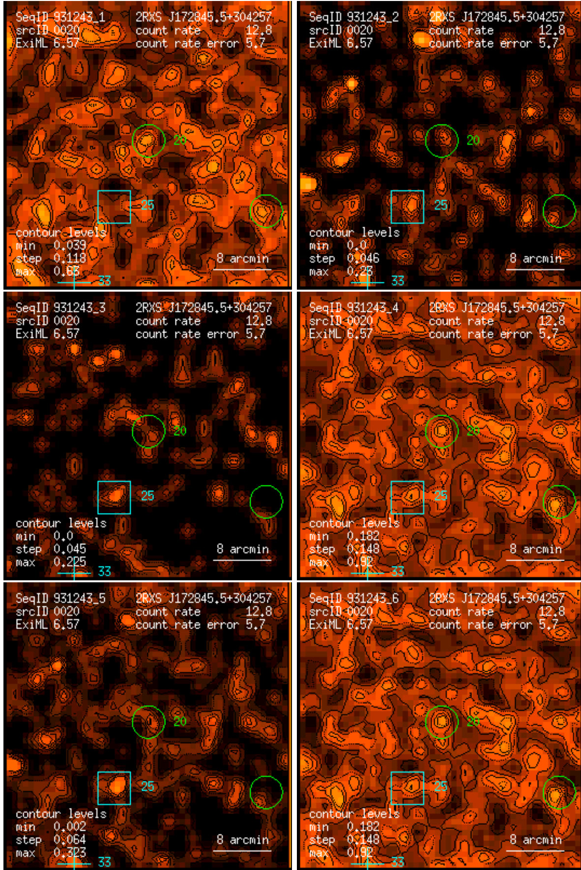
Figure 20: RASS 931243: detection 0020: band rate images, Gaussian filter: (1) PSPC channels 11 – 41, (2) 52 – 90, (3) 91 – 201, (4) 11 – 235, (5) 52 – 201, (6) 11 – 201. Broad band rates in counts/ks. Band rate contour levels in counts/ks/arcmin 2 .
