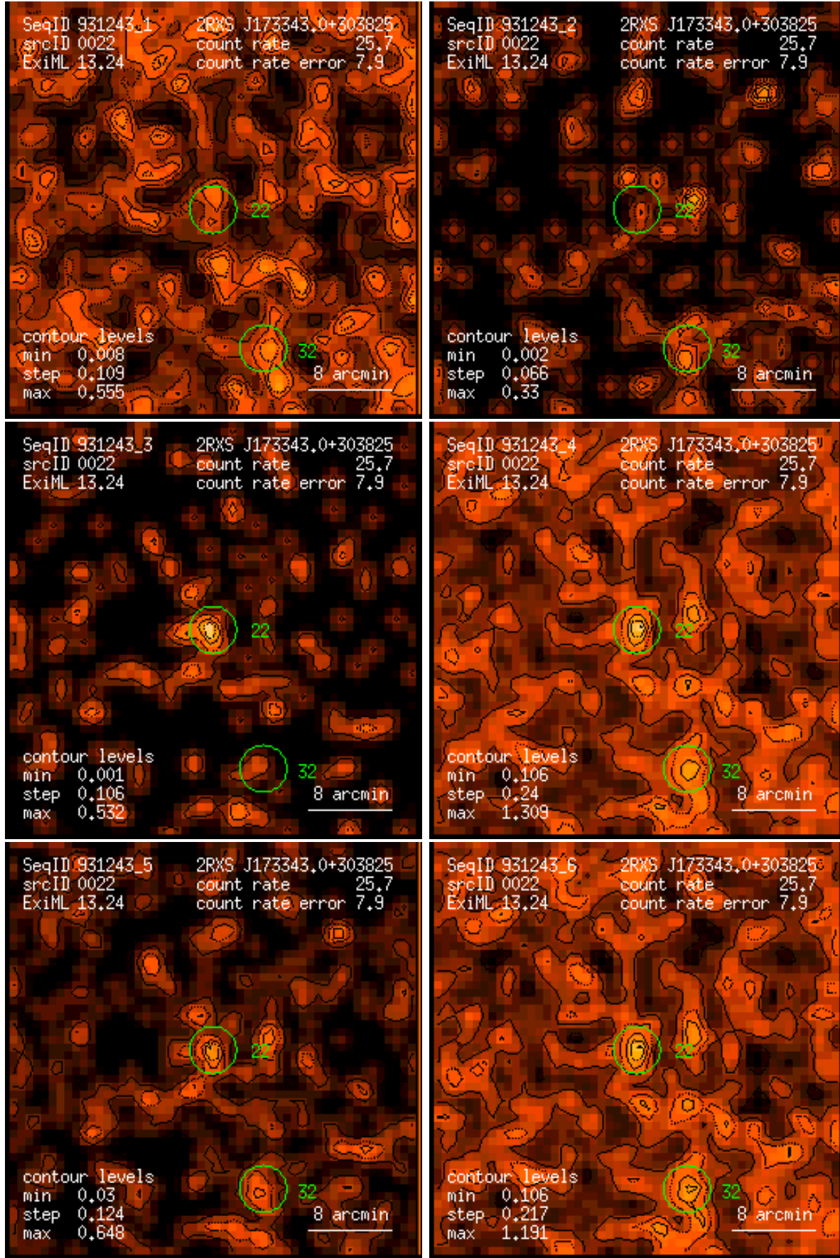
Figure 22: RASS 931243: detection 0022: band rate images, Gaussian filter: (1) PSPC channels 11 – 41, (2) 52 – 90, (3) 91 – 201, (4) 11 – 235, (5) 52 – 201, (6) 11 – 201. Broad band rates in counts/ks. Band rate contour levels in counts/ks/arcmin 2 .
