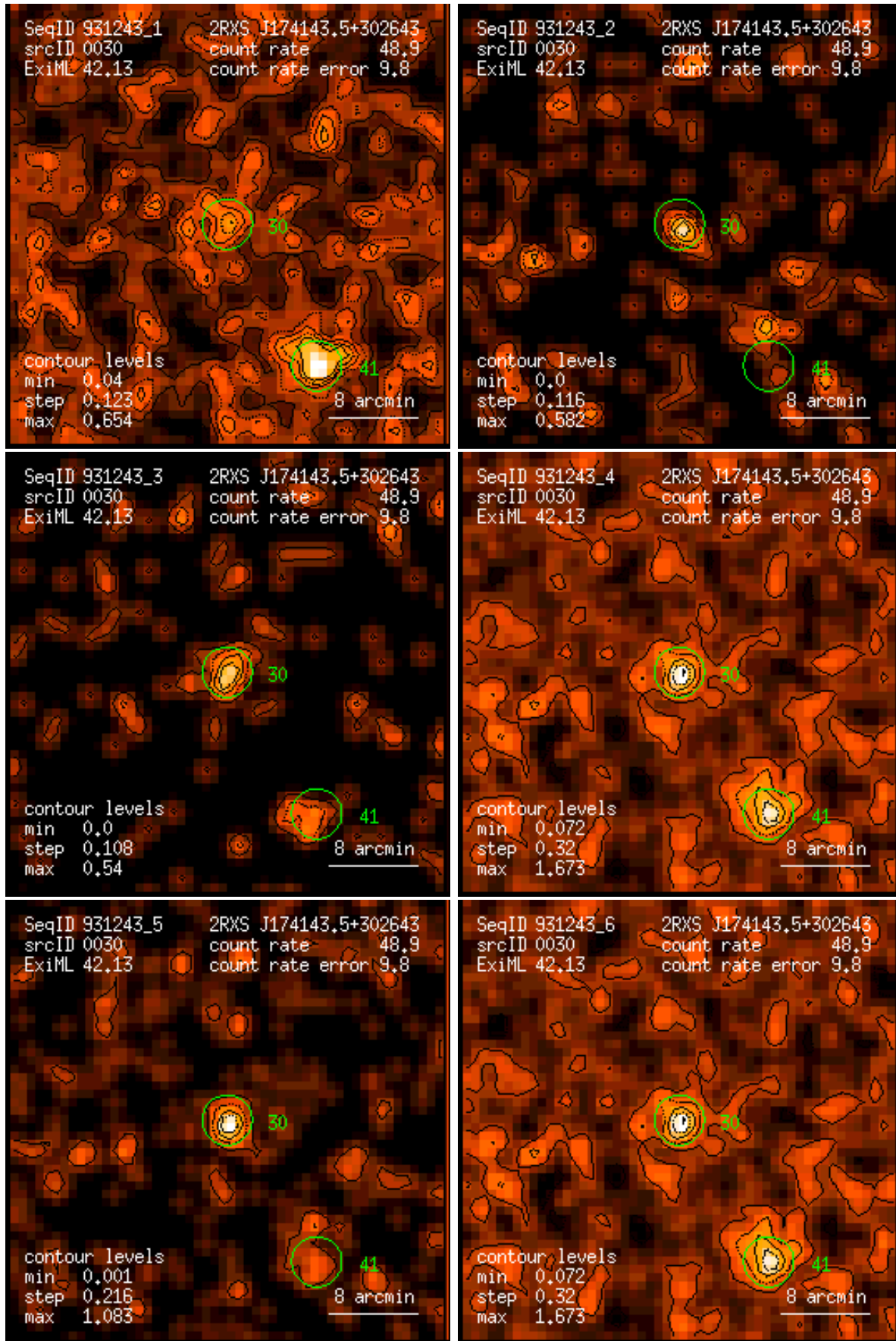
Figure 30: RASS 931243: detection 0030: band rate images, Gaussian filter: (1) PSPC channels 11 – 41, (2) 52 – 90, (3) 91 – 201, (4) 11 – 235, (5) 52 – 201, (6) 11 – 201. Broad band rates in counts/ks. Band rate contour levels in counts/ks/arcmin 2 .
