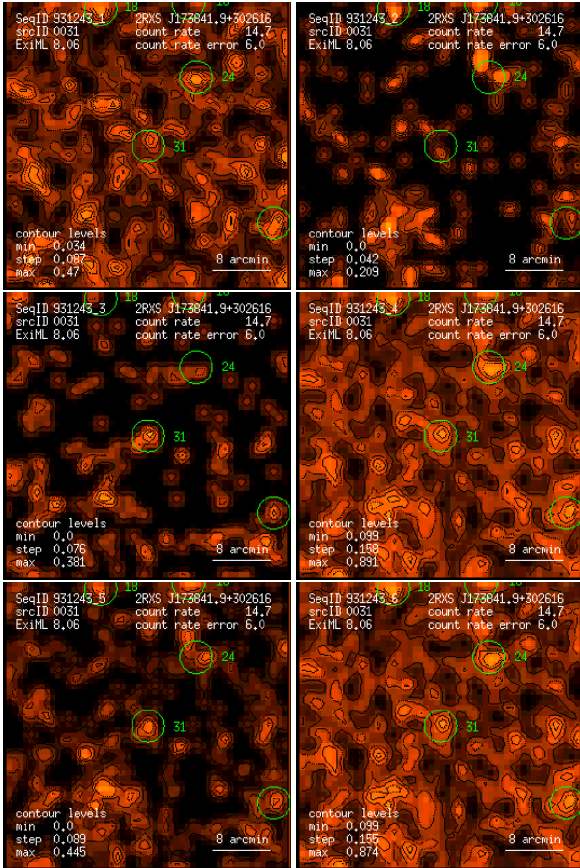
Figure 31: RASS 931243: detection 0031: band rate images, Gaussian filter: (1) PSPC channels 11 – 41, (2) 52 – 90, (3) 91 – 201, (4) 11 – 235, (5) 52 – 201, (6) 11 – 201. Broad band rates in counts/ks. Band rate contour levels in counts/ks/arcmin 2 .
