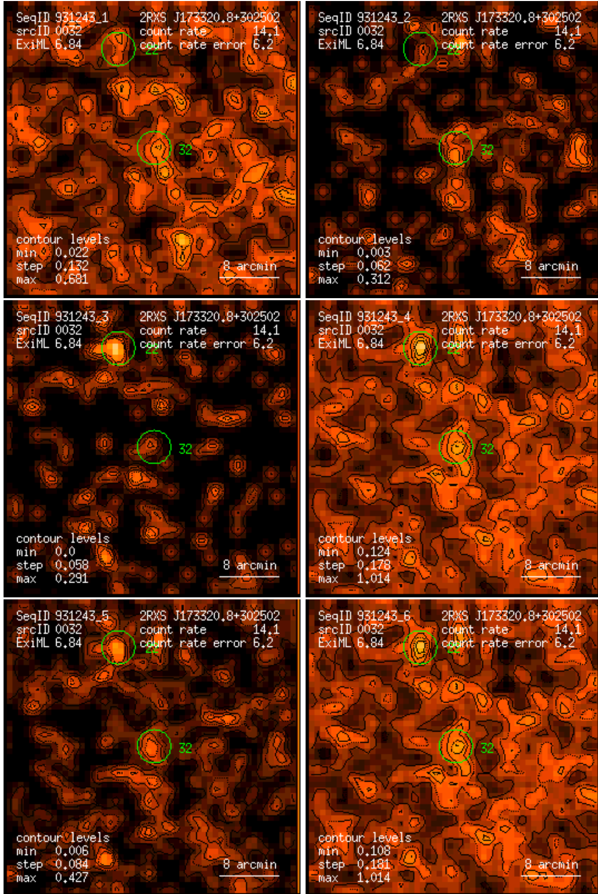
Figure 32: RASS 931243: detection 0032: band rate images, Gaussian filter: (1) PSPC channels 11 – 41, (2) 52 – 90, (3) 91 – 201, (4) 11 – 235, (5) 52 – 201, (6) 11 – 201. Broad band rates in counts/ks. Band rate contour levels in counts/ks/arcmin 2 .
