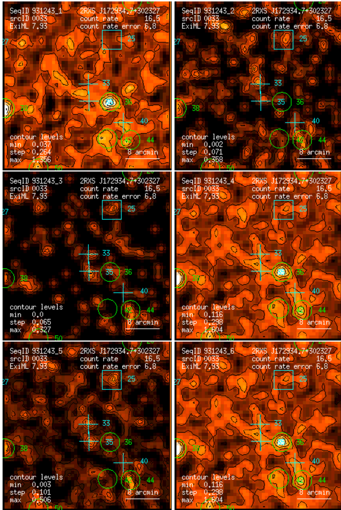
Figure 33: RASS 931243: detection 0033: band rate images, Gaussian filter: (1) PSPC channels 11 – 41, (2) 52 – 90, (3) 91 – 201, (4) 11 – 235, (5) 52 – 201, (6) 11 – 201. Broad band rates in counts/ks. Band rate contour levels in counts/ks/arcmin 2 .
