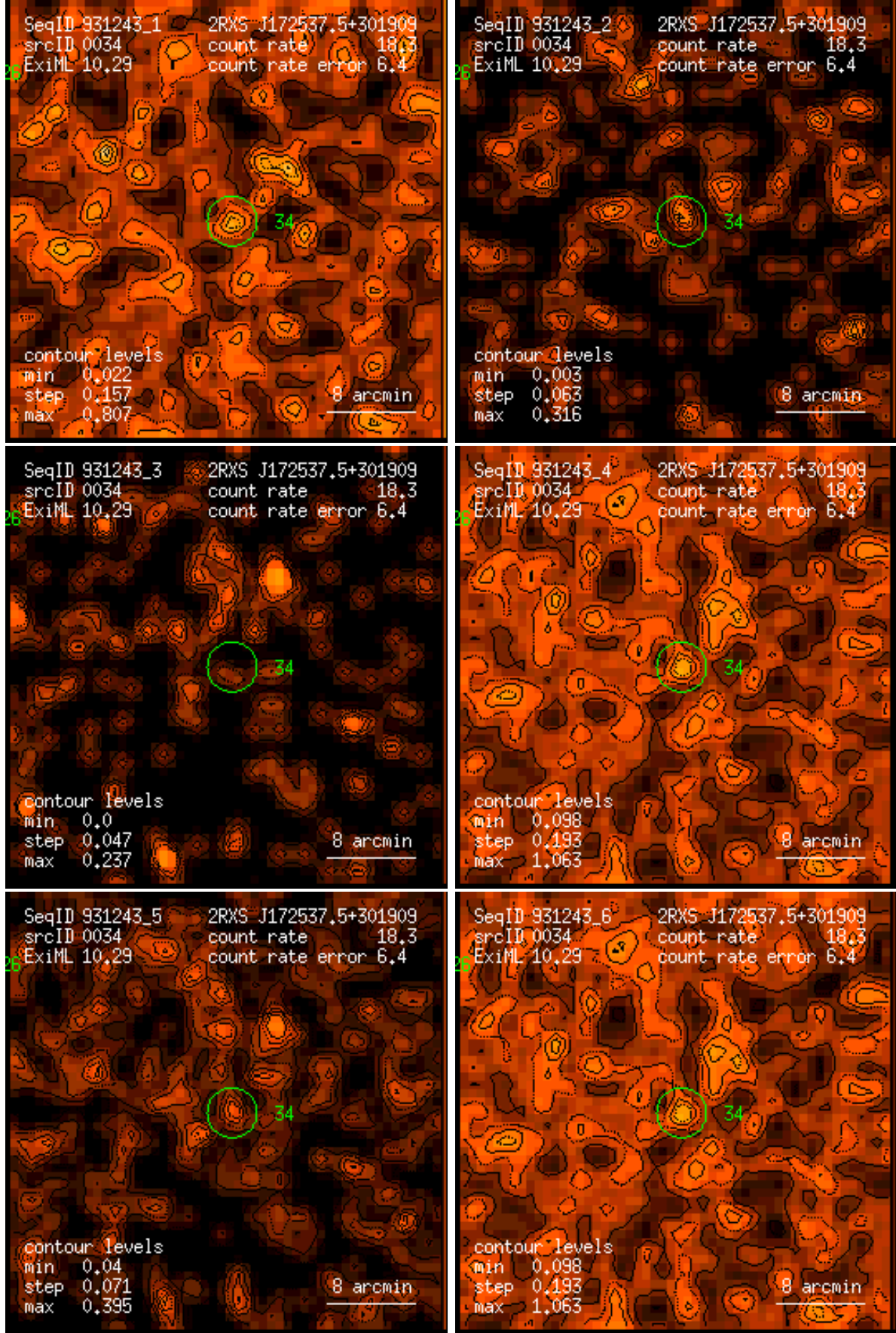
Figure 34: RASS 931243: detection 0034: band rate images, Gaussian filter: (1) PSPC channels 11 – 41, (2) 52 – 90, (3) 91 – 201, (4) 11 – 235, (5) 52 – 201, (6) 11 – 201. Broad band rates in counts/ks. Band rate contour levels in counts/ks/arcmin 2 .
