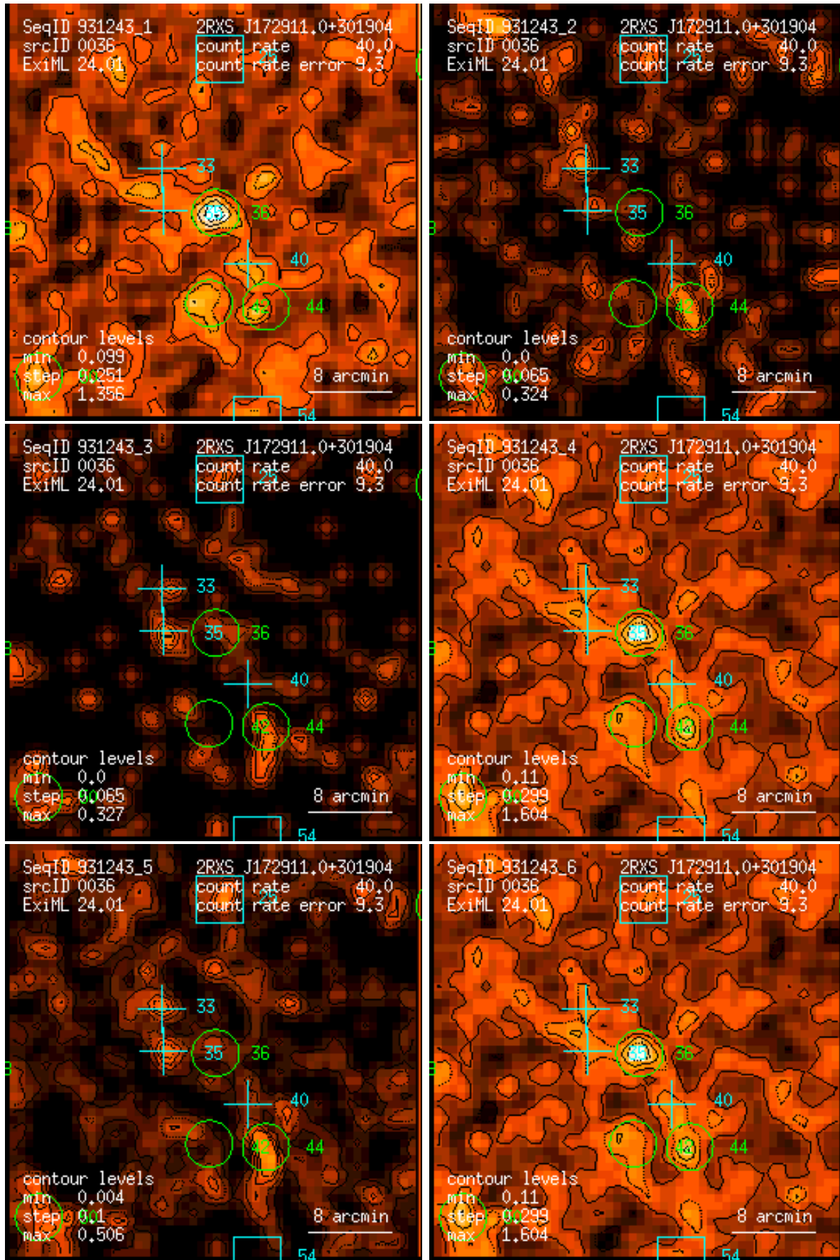
Figure 36: RASS 931243: detection 0036: band rate images, Gaussian filter: (1) PSPC channels 11 – 41, (2) 52 – 90, (3) 91 – 201, (4) 11 – 235, (5) 52 – 201, (6) 11 – 201. Broad band rates in counts/ks. Band rate contour levels in counts/ks/arcmin 2 .
