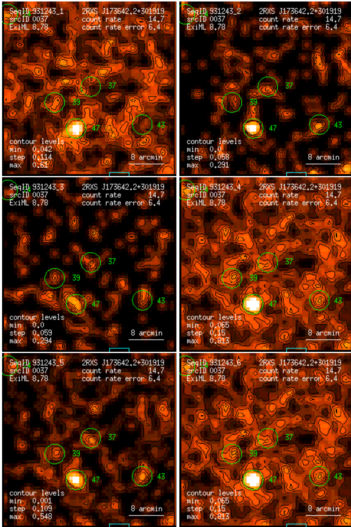
Figure 37: RASS 931243: detection 0037: band rate images, Gaussian filter: (1) PSPC channels 11 – 41, (2) 52 – 90, (3) 91 – 201, (4) 11 – 235, (5) 52 – 201, (6) 11 – 201. Broad band rates in counts/ks. Band rate contour levels in counts/ks/arcmin 2 .
