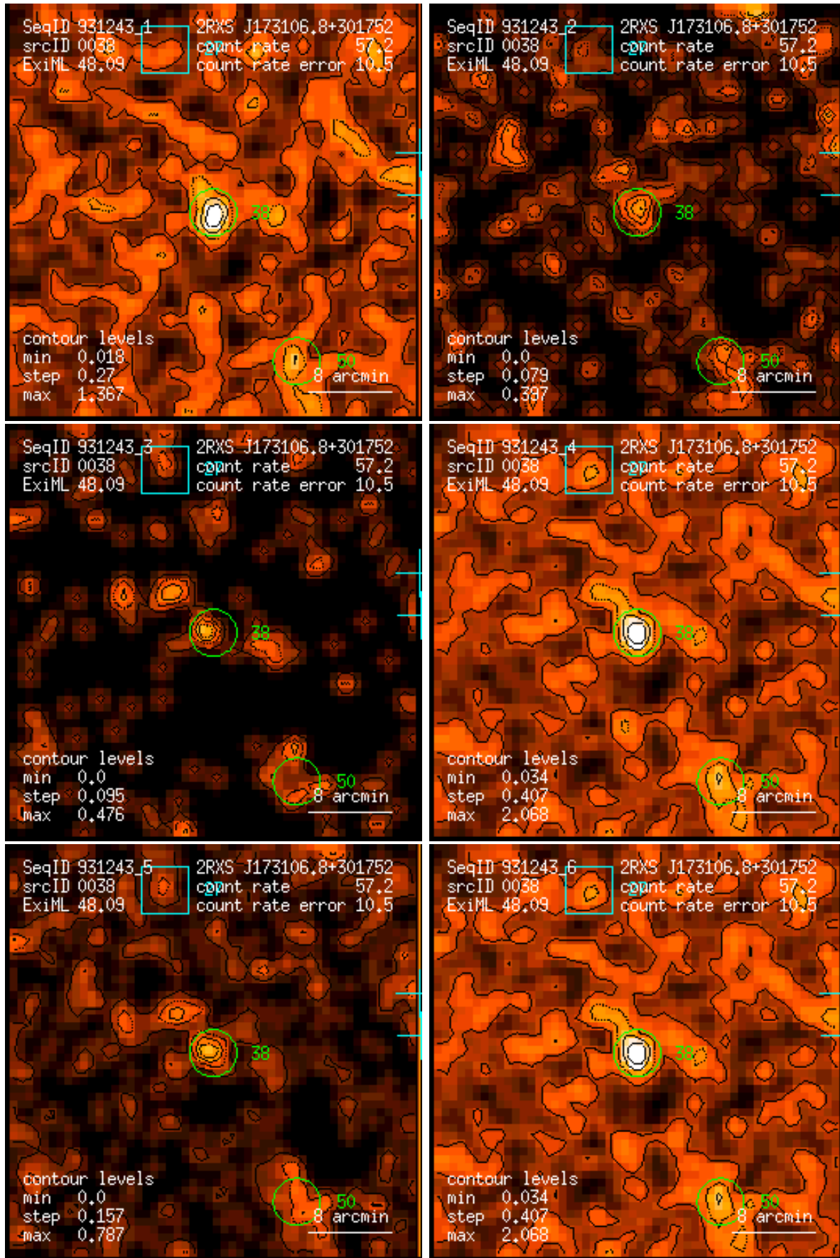
Figure 38: RASS 931243: detection 0038: band rate images, Gaussian filter: (1) PSPC channels 11 – 41, (2) 52 – 90, (3) 91 – 201, (4) 11 – 235, (5) 52 – 201, (6) 11 – 201. Broad band rates in counts/ks. Band rate contour levels in counts/ks/arcmin 2 .
