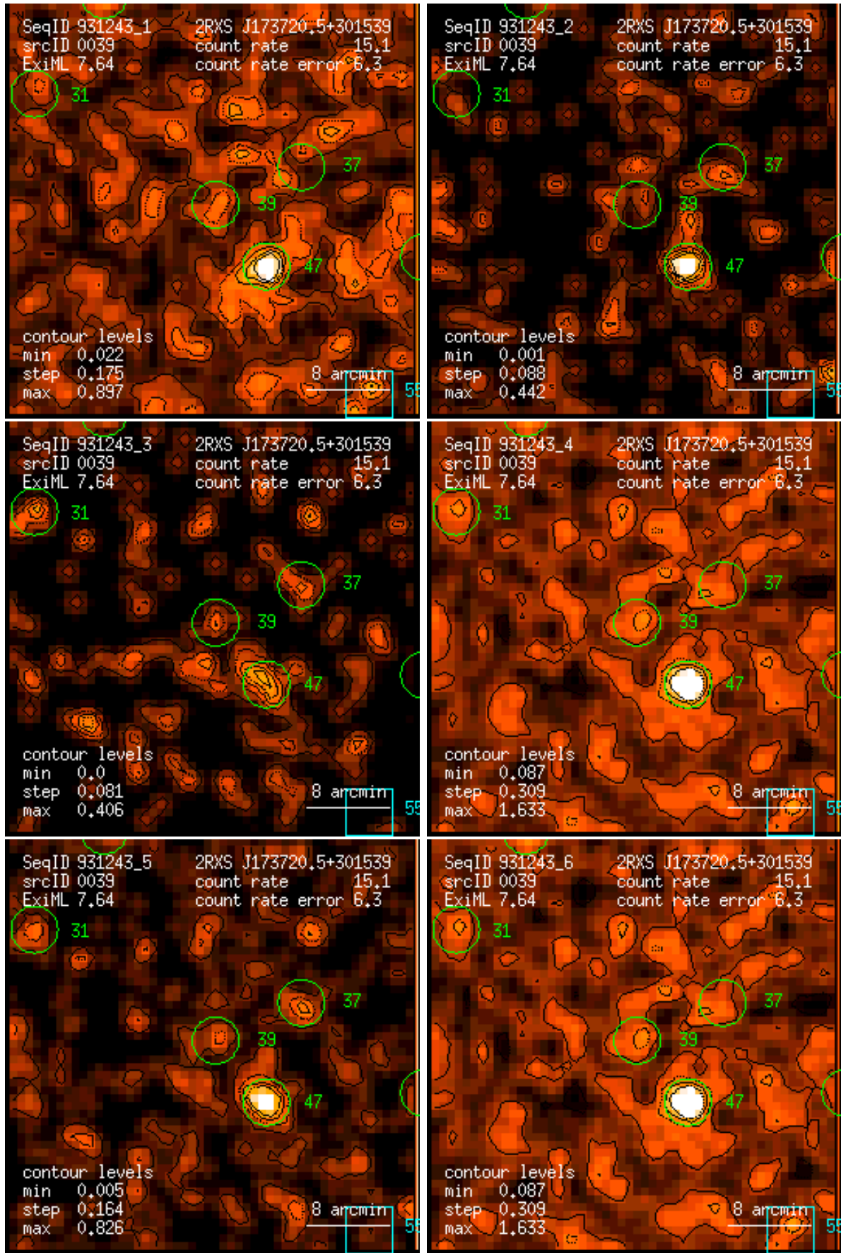
Figure 39: RASS 931243: detection 0039: band rate images, Gaussian filter: (1) PSPPC channels 11 – 41, (2) 52 – 90, (3) 91 – 201, (4) 11 – 235, (5) 52 – 201, (6) 11 – 201. Broad band rates in counts/ks. Band rate contour levels in counts/ks/arcmin 2 .
