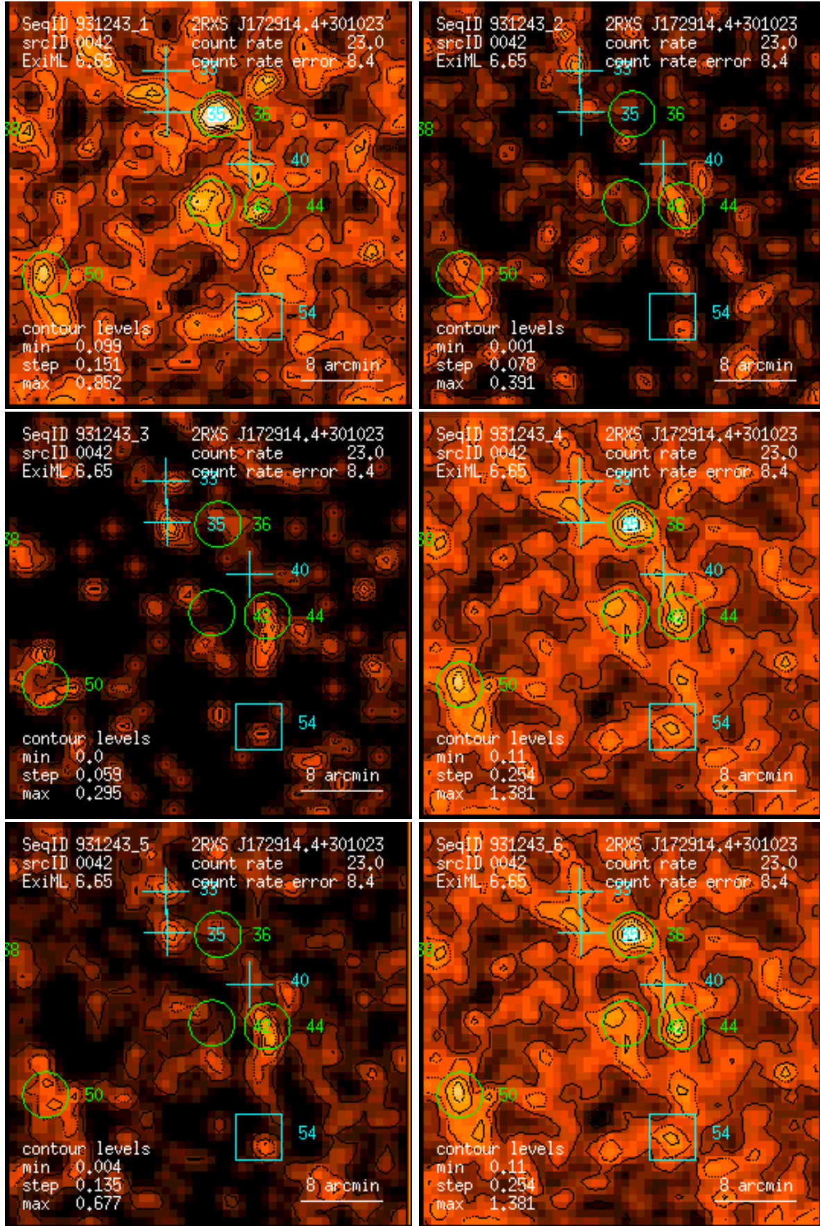
Figure 42: RASS 931243: detection 0042: band rate images, Gaussian filter: (1) PSPC channels 11 – 41, (2) 52 – 90, (3) 91 – 201, (4) 11 – 235, (5) 52 – 201, (6) 11 – 201. Broad band rates in counts/ks. Band rate contour levels in counts/ks/arcmin 2 .
