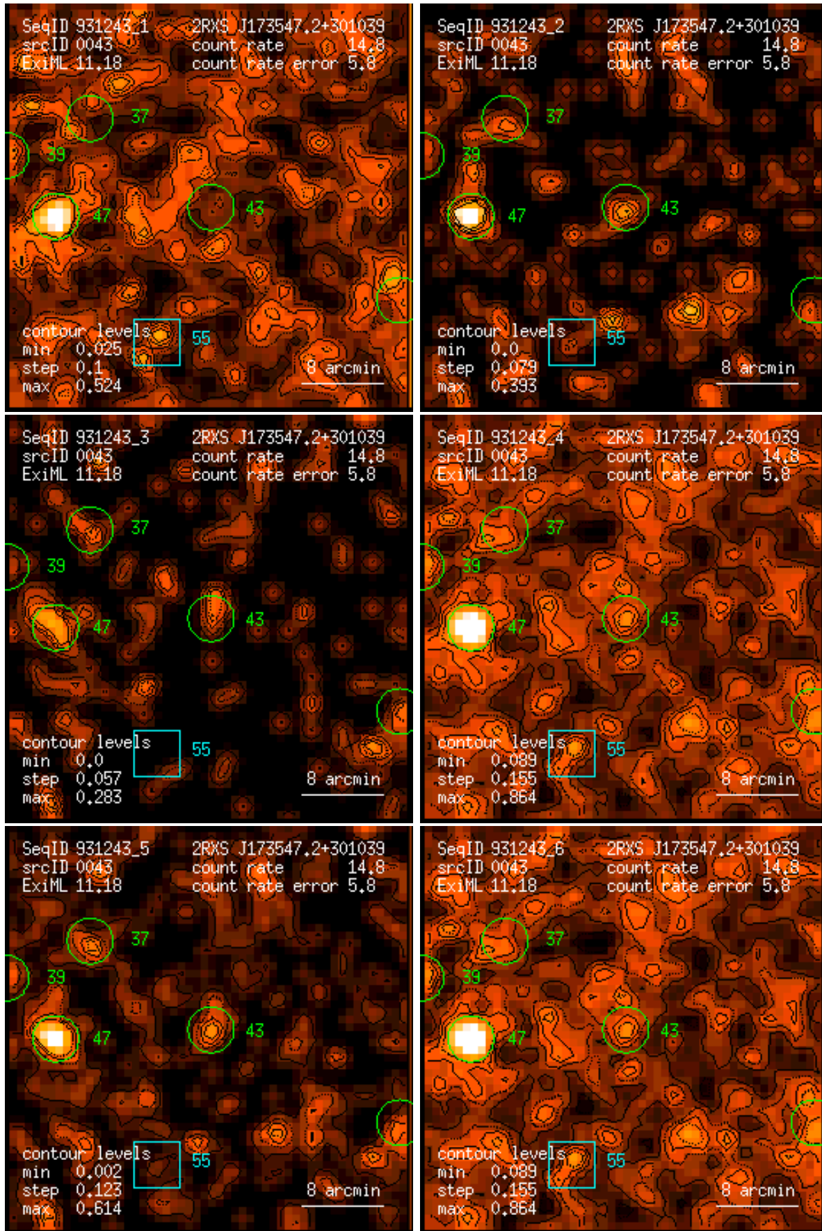
Figure 43: RASS 931243: detection 0043: band rate images, Gaussian filter: (1) PSPC channels 11 – 41, (2) 52 – 90, (3) 91 – 201, (4) 11 – 235, (5) 52 – 201, (6) 11 – 201. Broad band rates in counts/ks. Band rate contour levels in counts/ks/arcmin 2 .
