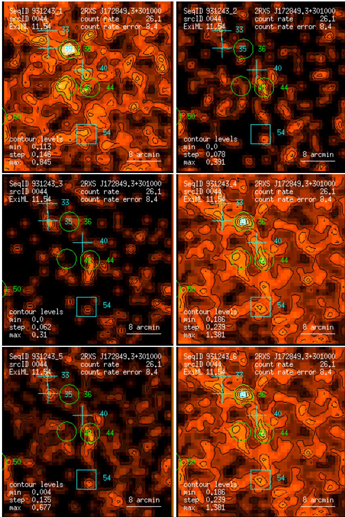
Figure 44: RASS 931243: detection 0044: band rate images, Gaussian filter: (1) PSPC channels 11 – 41, (2) 52 – 90, (3) 91 – 201, (4) 11 – 235, (5) 52 – 201, (6) 11 – 201. Broad band rates in counts/ks. Band rate contour levels in counts/ks/arcmin 2 .
